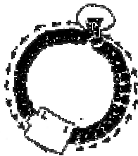
Fig. 4: Cyclic Simultaneous Causal Models
